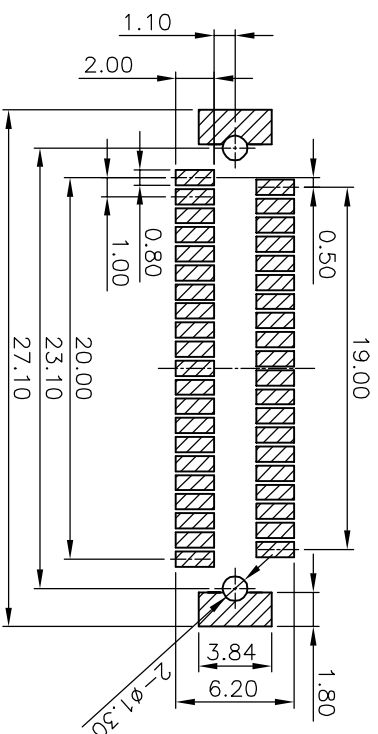
PCB LAYOUT TOP VIEW
